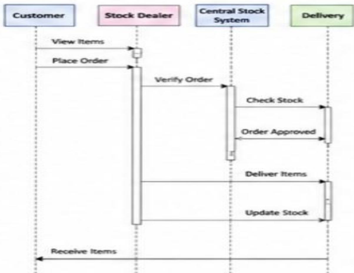
Sequence Diagram
