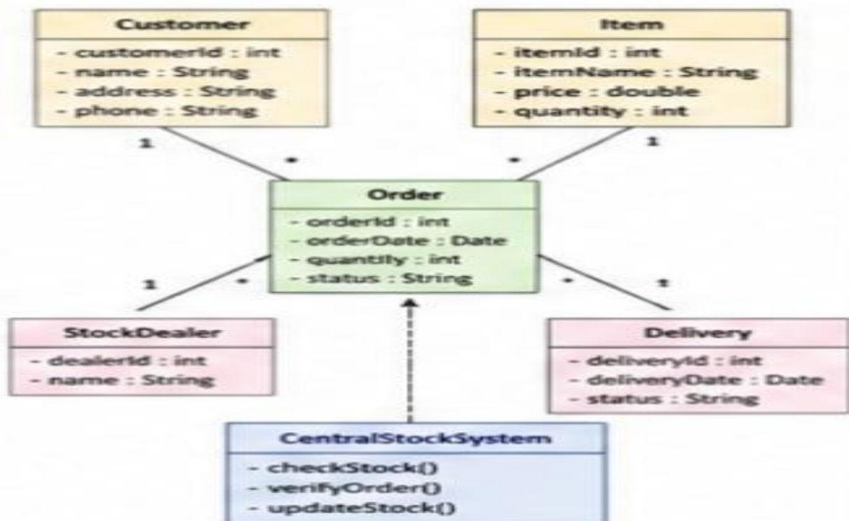
Class Diagram
